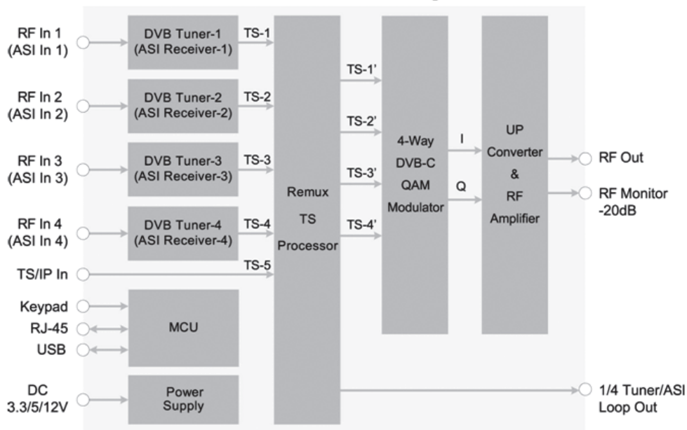
WDH-1540TM Functional Block Diagram
